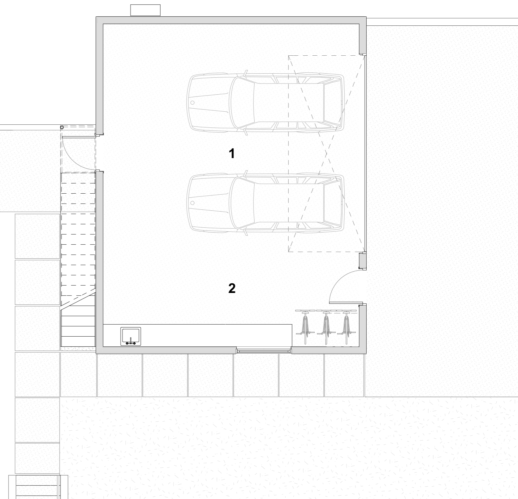
GARAGE/ DADU LEVEL 1
