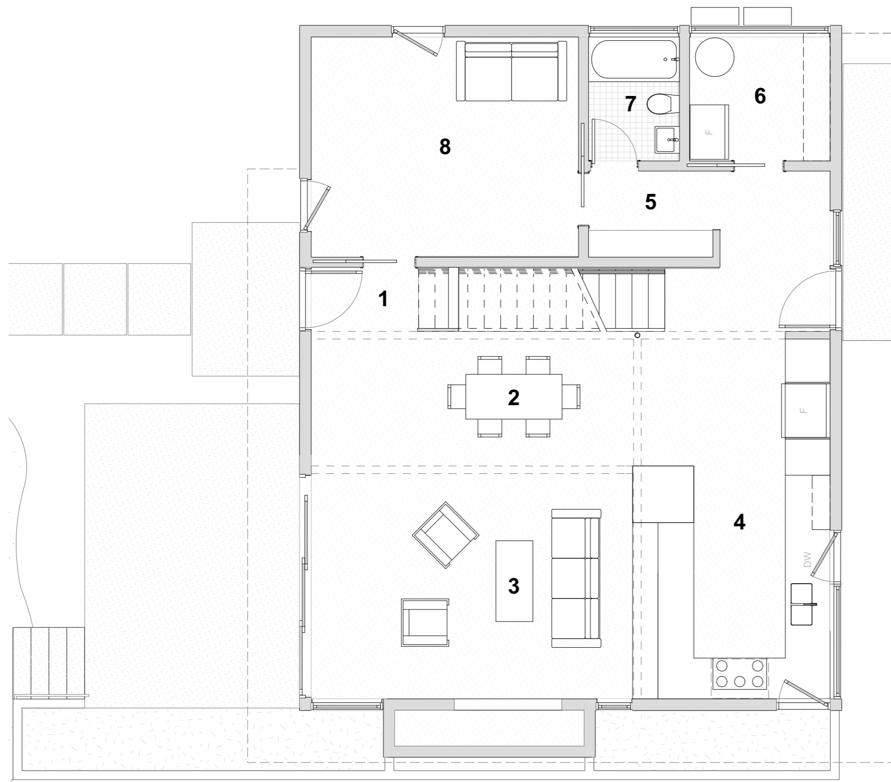
HOUSE LEVEL 1
