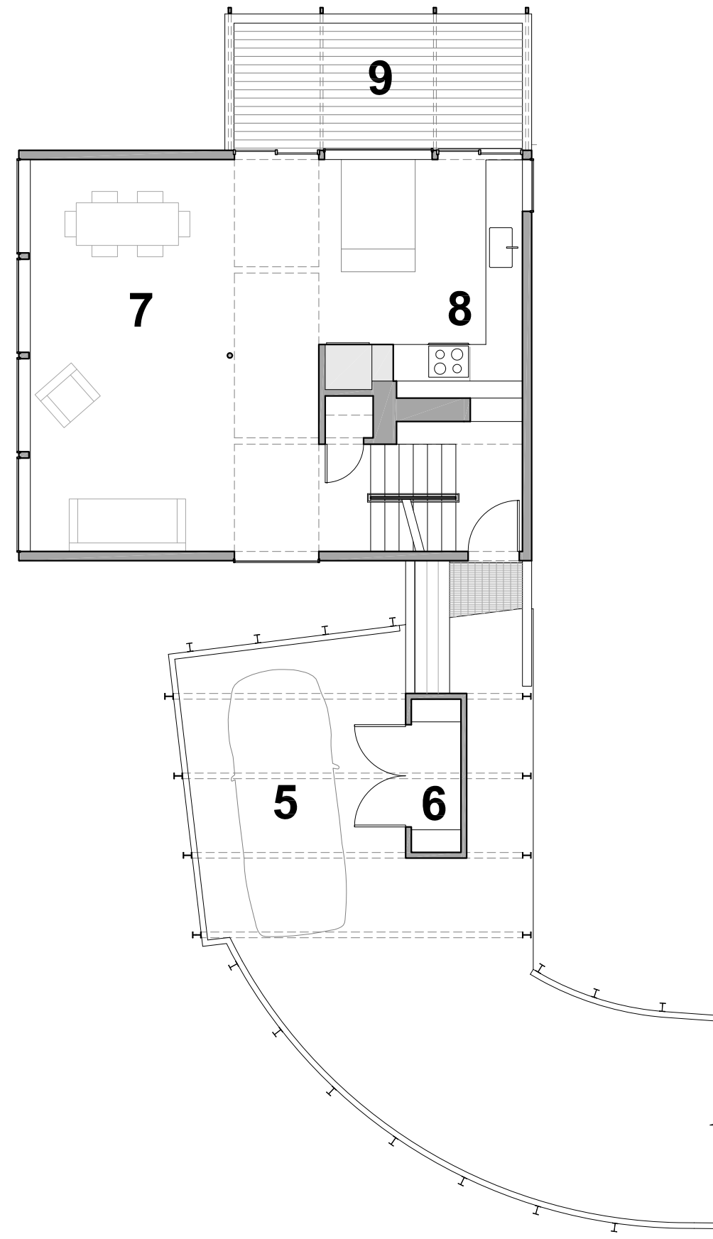
MAIN FLOOR
